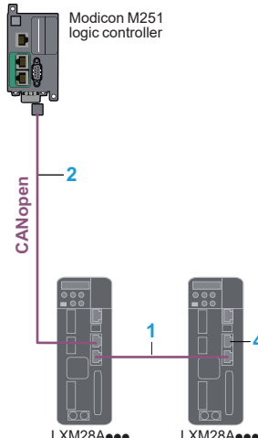
Examples of architectures with control by Modicon M241/M251 logic controllers or LMC058 motion controller
